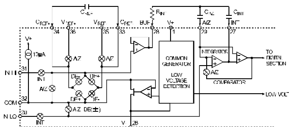
Figure4. Analog Section
