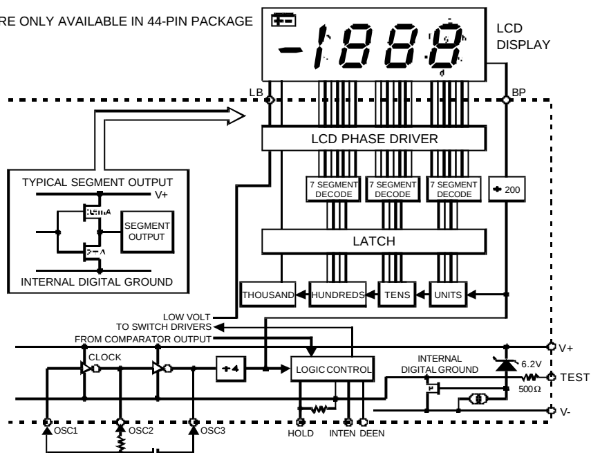
Figure7. AME7107 Digital Section
