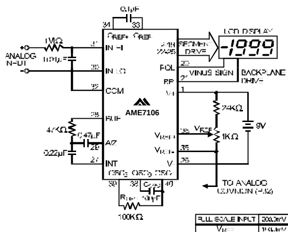
Figure1. AME7106 Typical Operating Circuit
