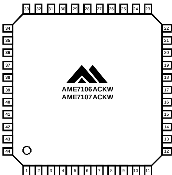
Figure3. Pin Configurations
