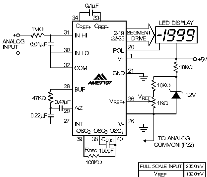
Figure12. Operating AME7107 from a single 5V Supply
