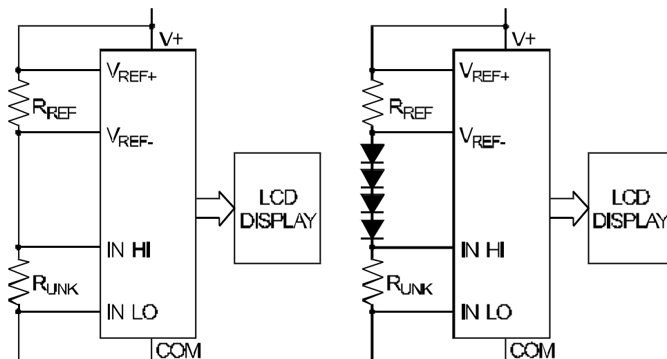
Figure11. Ratiometric Resistance Measurement
